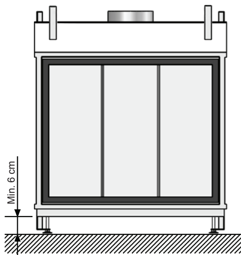
Figure 15: A clearance of at least 6 cm must be maintained between the bottom plate of the appliance and the floor.
