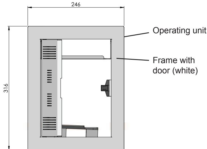
Figure 18: Operating unit
